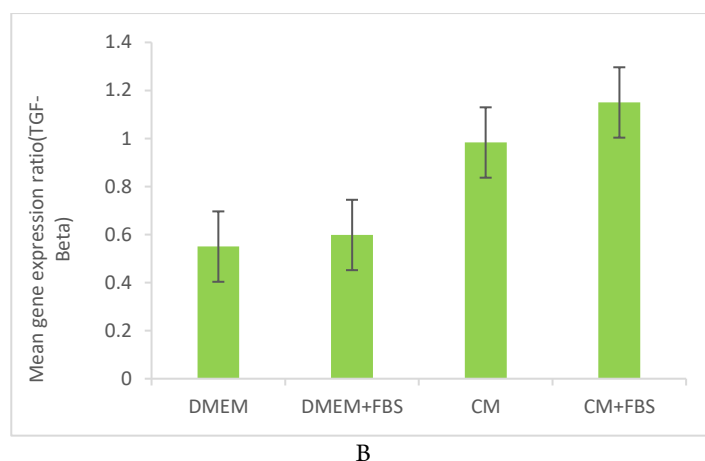
Figure 4. Relative expression analysis of TGF- \beta using qRT-PCR in A431 (A) and HDF-a (B). Elevated expression of TGF- \beta in cells treated with CM compared with DMEM and DMEM with FBS. Results are the mean \pm SEM. Each test was repeated three times. * P < 0.05
